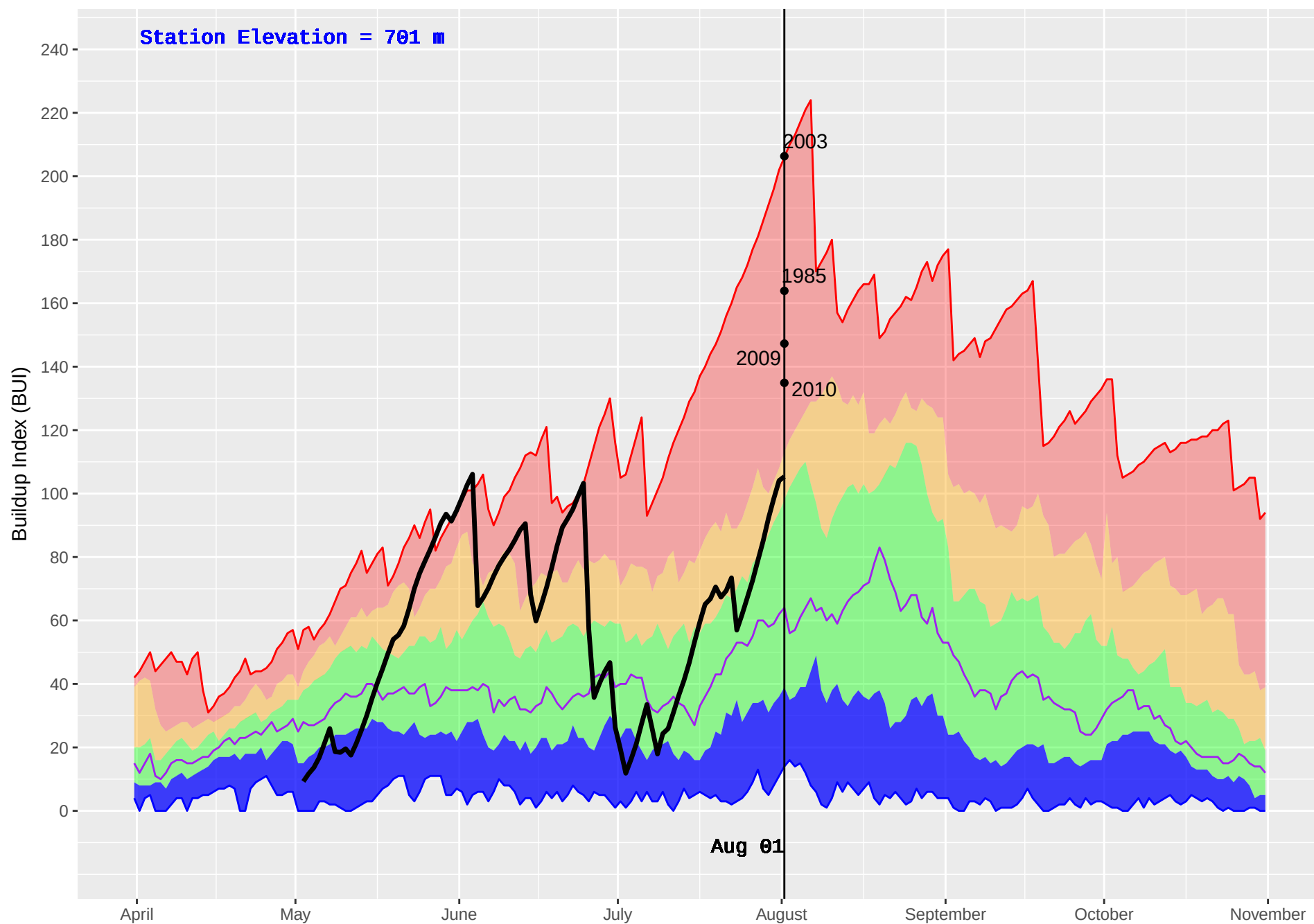
HORSEFLY (230) : Historical (1971–2016) and Current (2018) Daily Buildup Index (BUI)
