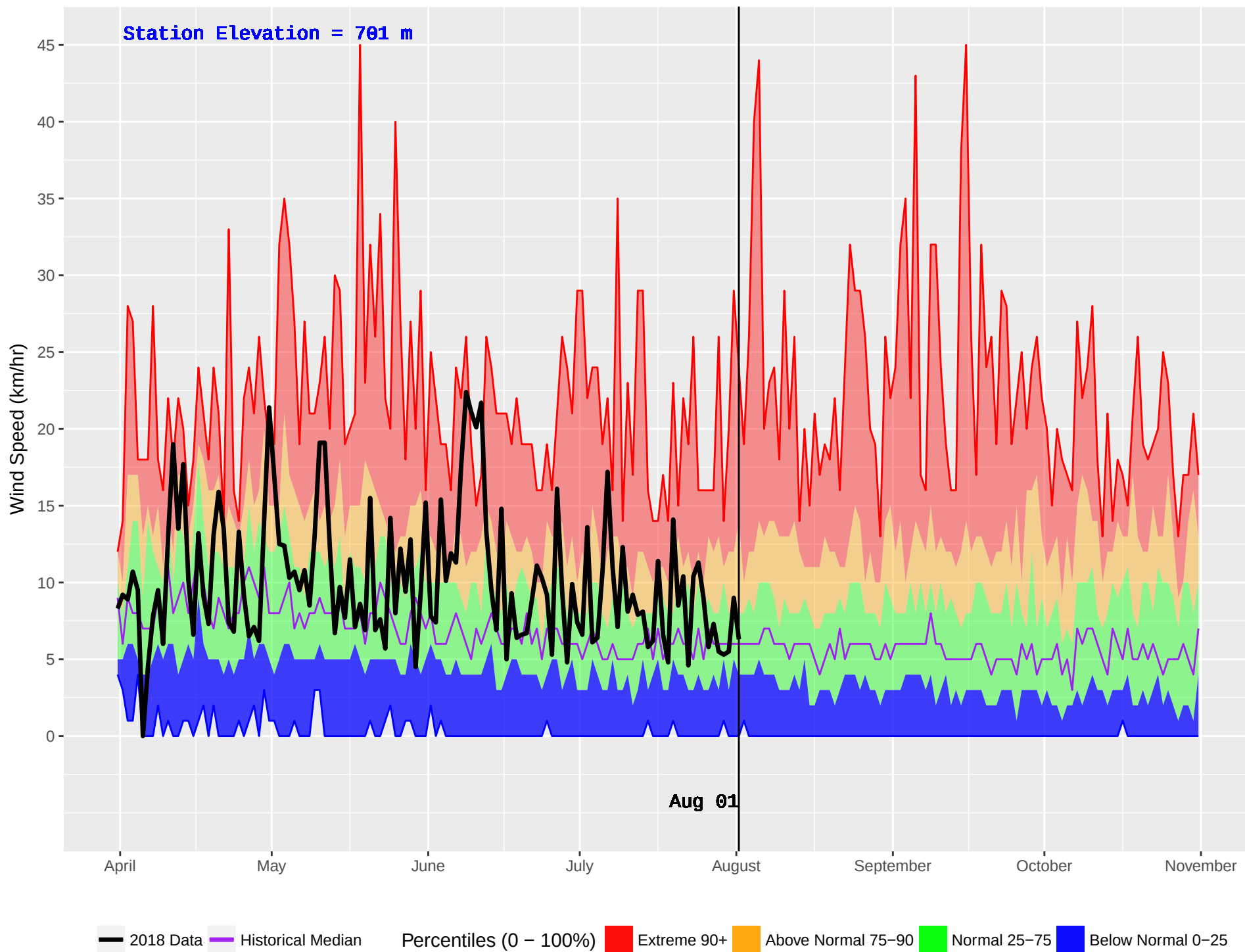
HORSEFLY (230) : Historical (1971–2016) and Current (2018) Daily Wind Speed
